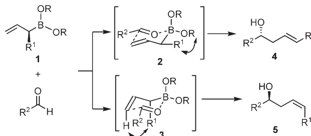
Scheme 1. Competing transition structures in the allylation of aldehydes with chiral \alpha -substituted allylboronates ( 1 ).
